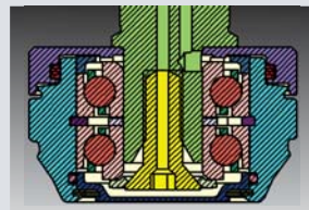
Flow-Thru Lubrication with Ceramic Balls and Labyrinth Seal
