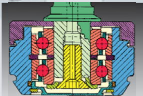
Angular Contact Bearing with Ceramic Balls
