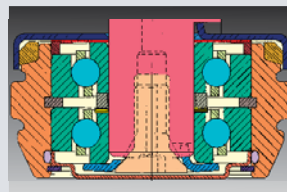
Non Flow-Thru Lubrication with Ceramic Balls
