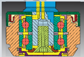
Flow-Thru Lubrication with Ceramic Balls
