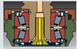
Flow-Thru Lubrication with Tapered Roller and Labyrinth Seal
